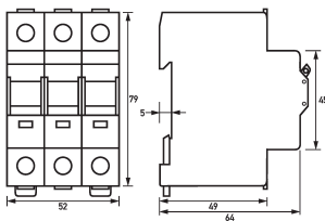
Dimensional drawing Group view
